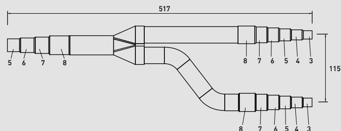
Lato gas
