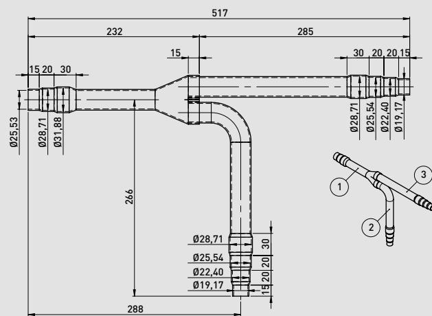
Lato gas
